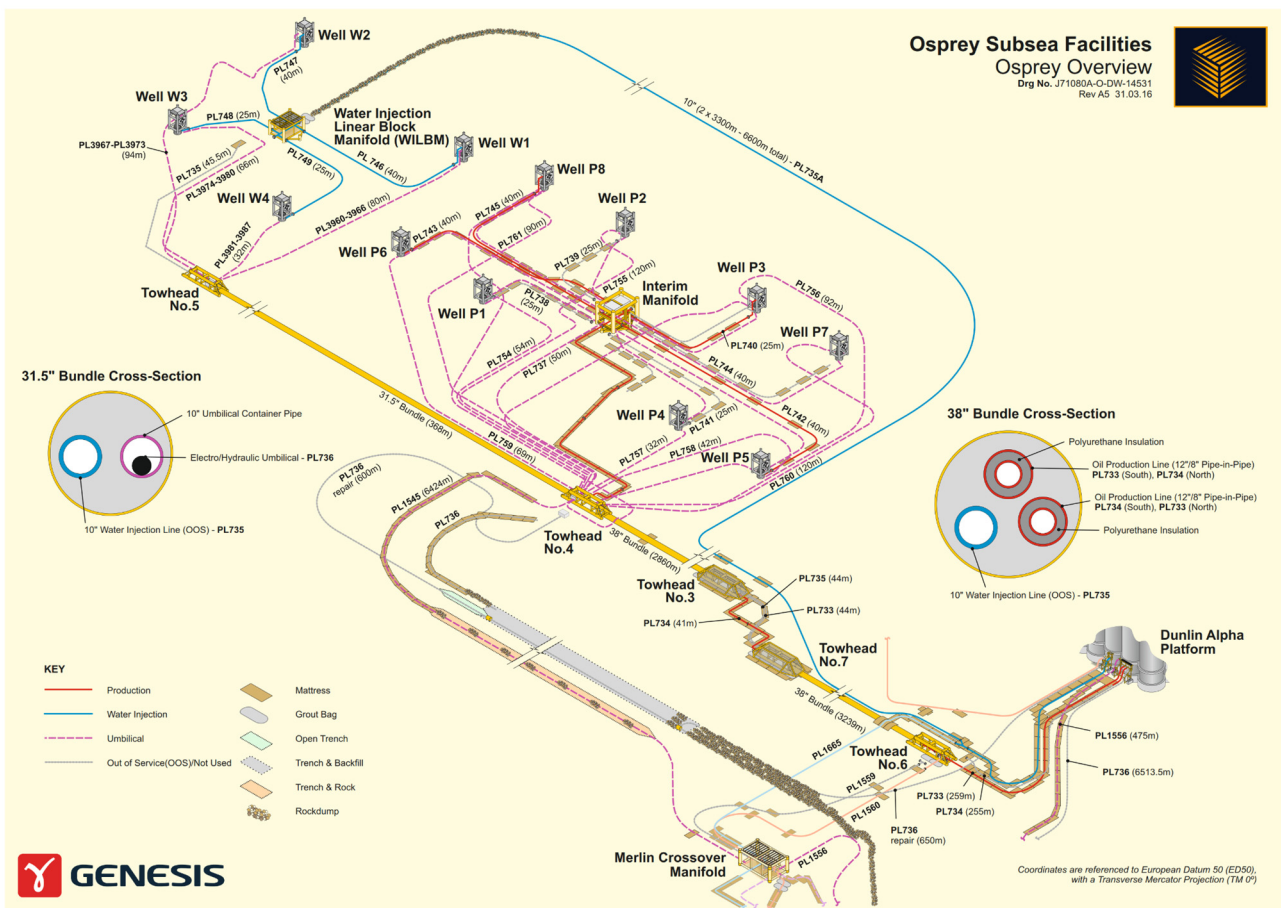
Figure 2.1 Osprey subsea facilities schematic
