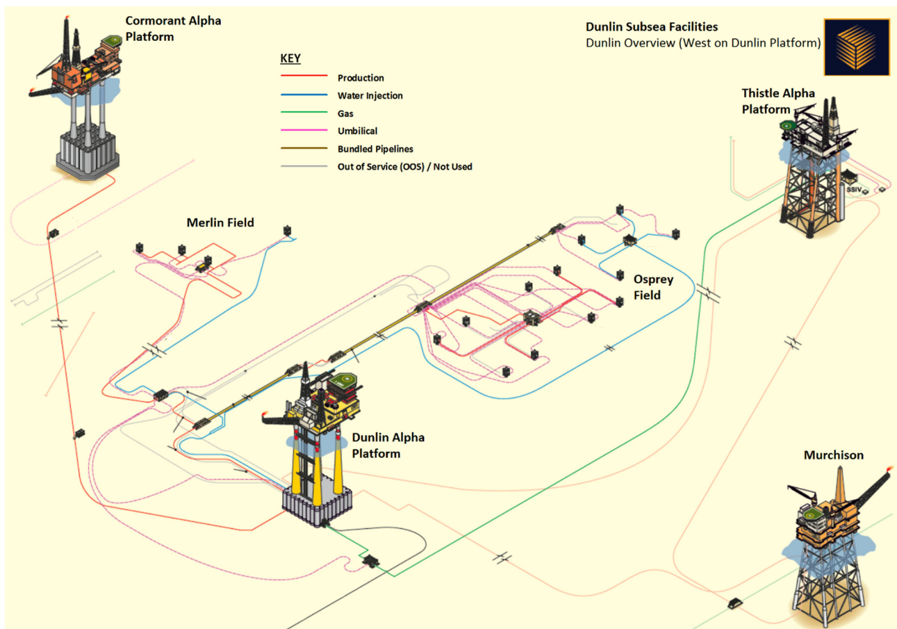
Figure 1.2 Osprey field infrastructure in the context of the wider area
