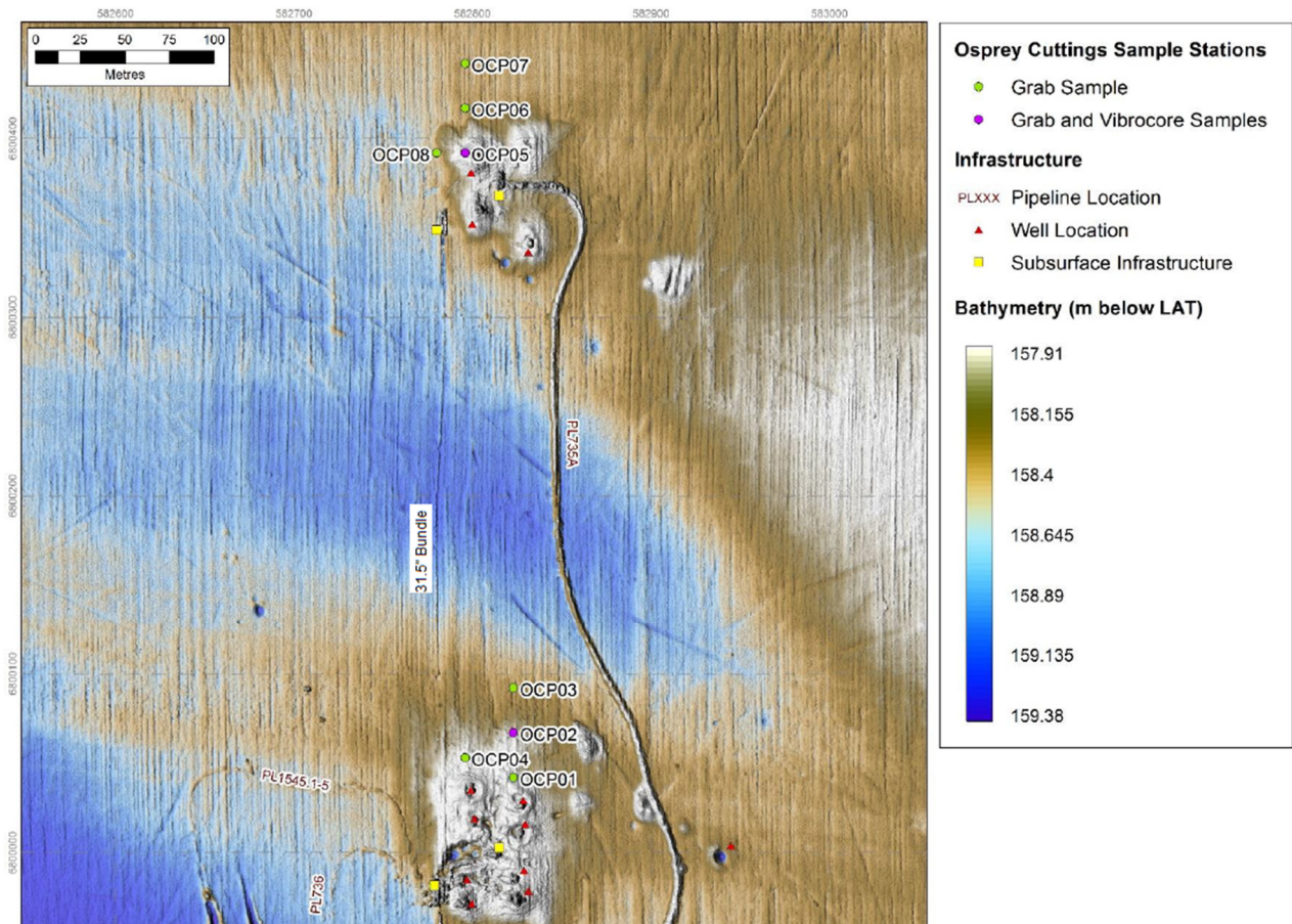
Figure 2.3 Osprey wells and drill cuttings (Fugro, 2017)
