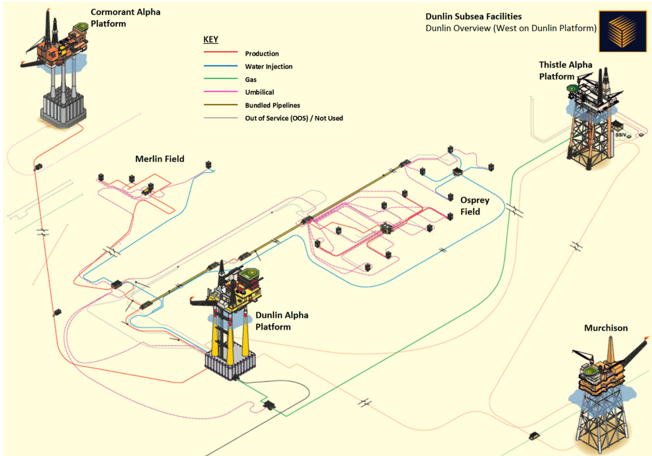
Figure 2 Osprey field infrastructure in the context of the wider area
