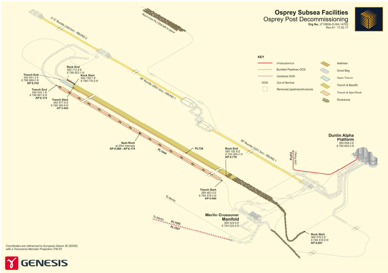
Figure 8 Subsea layout after completion of the decommissioning activities
