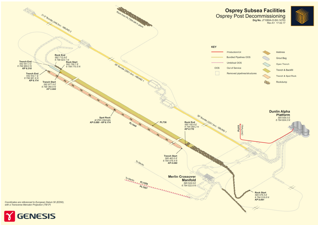
Figure 2.9 Subsea layout after completion of the decommissioning activities
